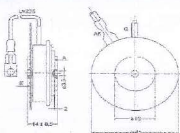
OUTLINE DIAGRAM-13
