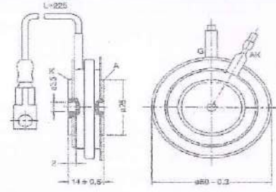
OUTLINE DIAGRAM-14
