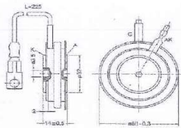
OUTLINE DIAGRAM-13
