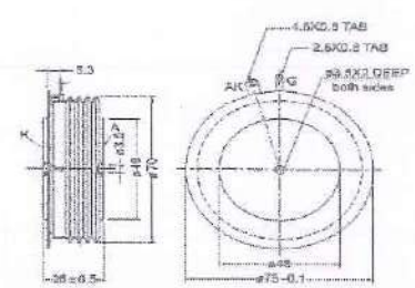
OUTLINE DIAGRAM-14
